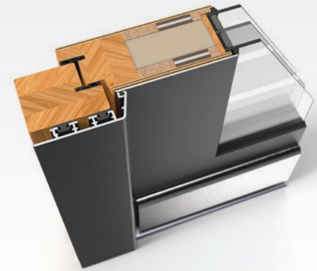
SOFT Outside lining of the door leaf and frame in aluminium
